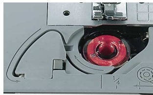
QUICK-SET BOBBIN
